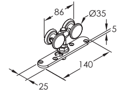
No. 57KN or No. 57KS HANGER
