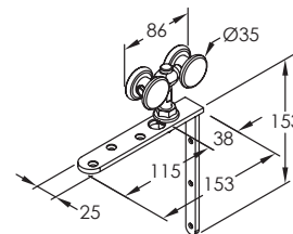
No. 52KN HANGER
