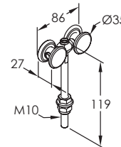
No. 56KLN or No. 56KLS HANGER
