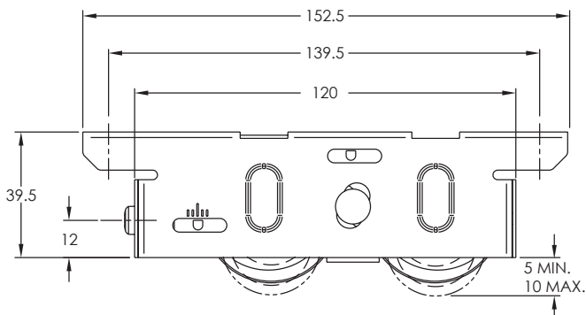
913DBA-300N END ADJUSTABLE ROLLER
