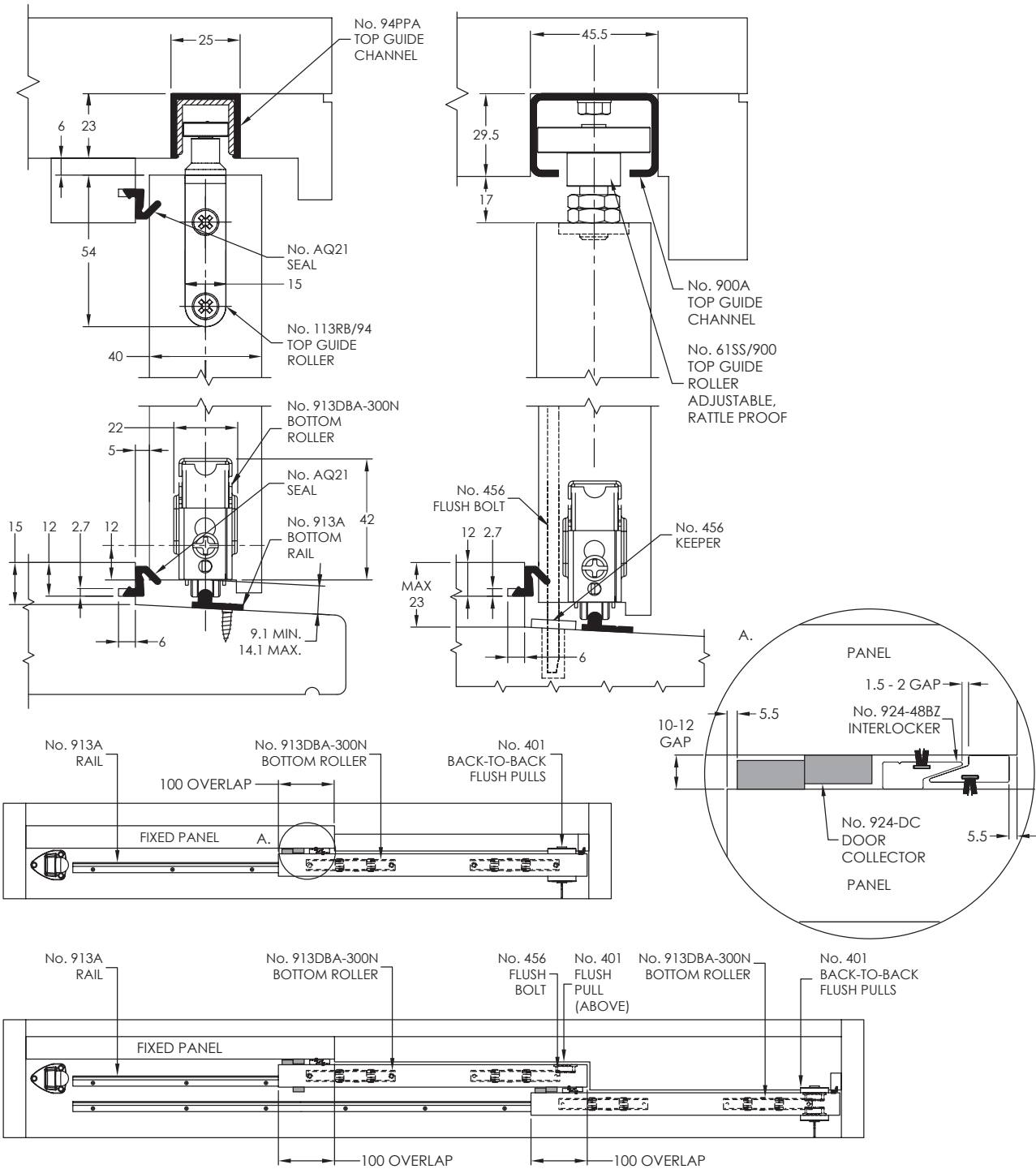
913DBA-300N END ADJUSTABLE ROLLER
